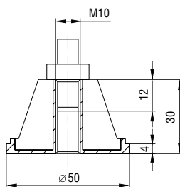
Опора D50M с гайкой M10 Support art. D50M with nut M10
