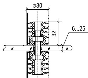
Опора П30 Support art. P30
